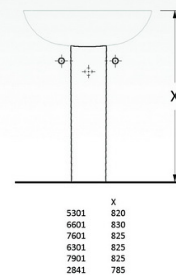
• F005 Ortak Tam Ayak • 5301, 6601, 7601, 6301, 7901, 2841 Lavabo
